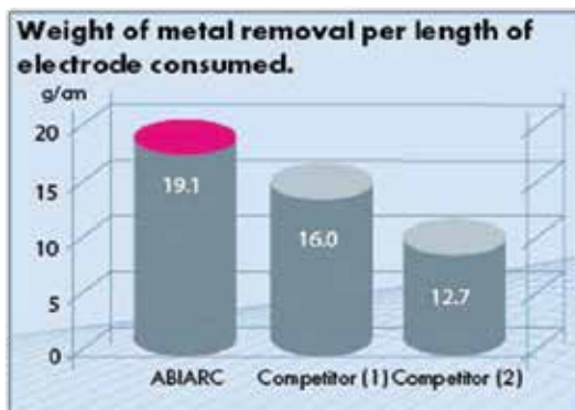
ABIARC Gouging electrodes (DC) pointed
