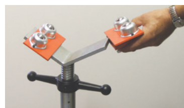
Slip on style heads
